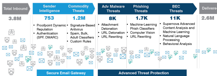
Message counts for attachment and URL threats across an organization's clusters
